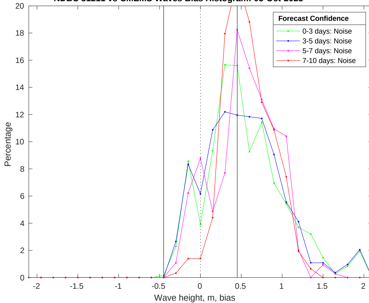
NDBC 51211 vs CMEMS Waves Bias Histogram: 03-Oct-2025
