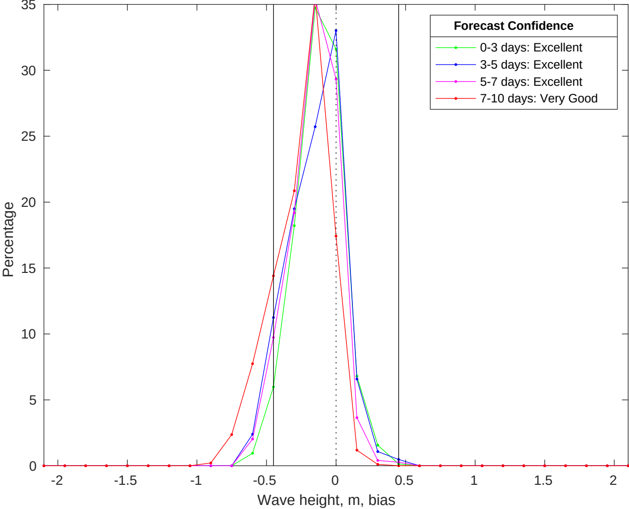
NDBC 52213 vs CMEMS Waves Bias Histogram: 03-Oct-2025
