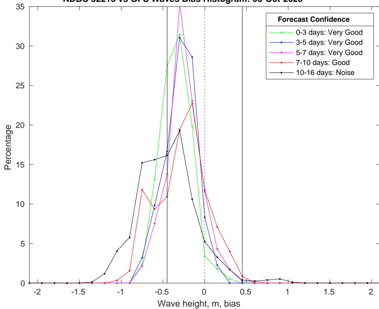
NDBC 52213 vs GFS Waves Bias Histogram: 03-Oct-2025
