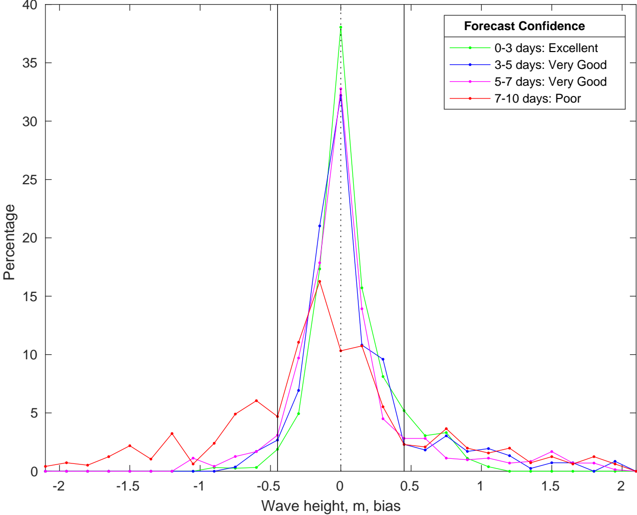
NDBC 41004 vs CMEMS Waves Bias Histogram: 04-Oct-2025
