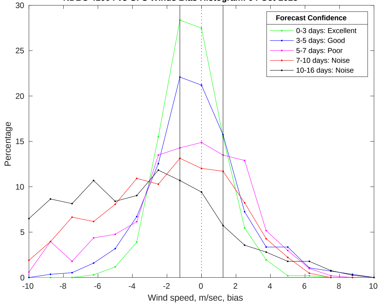
NDBC 41004 vs GFS Winds Bias Histogram: 04-Oct-2025
