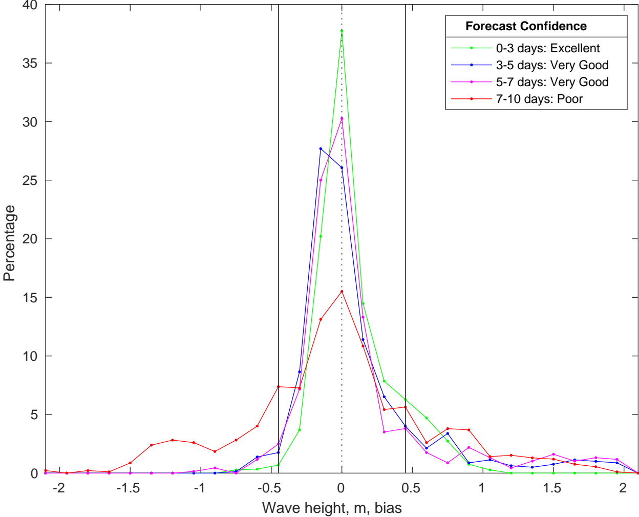
NDBC 41013 vs CMEMS Waves Bias Histogram: 04-Oct-2025
