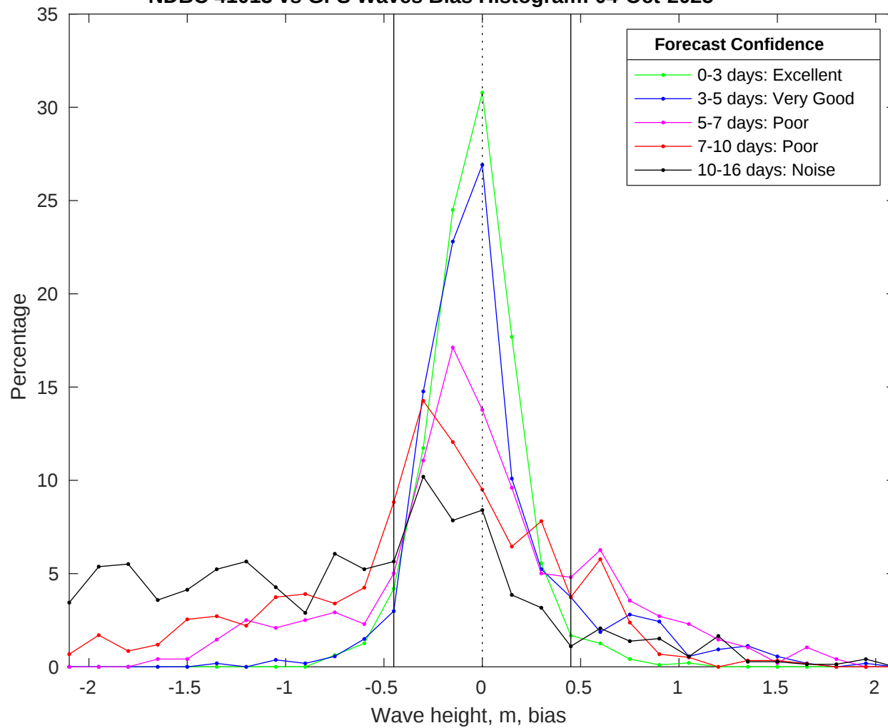
NDBC 41013 vs GFS Waves Bias Histogram: 04-Oct-2025
