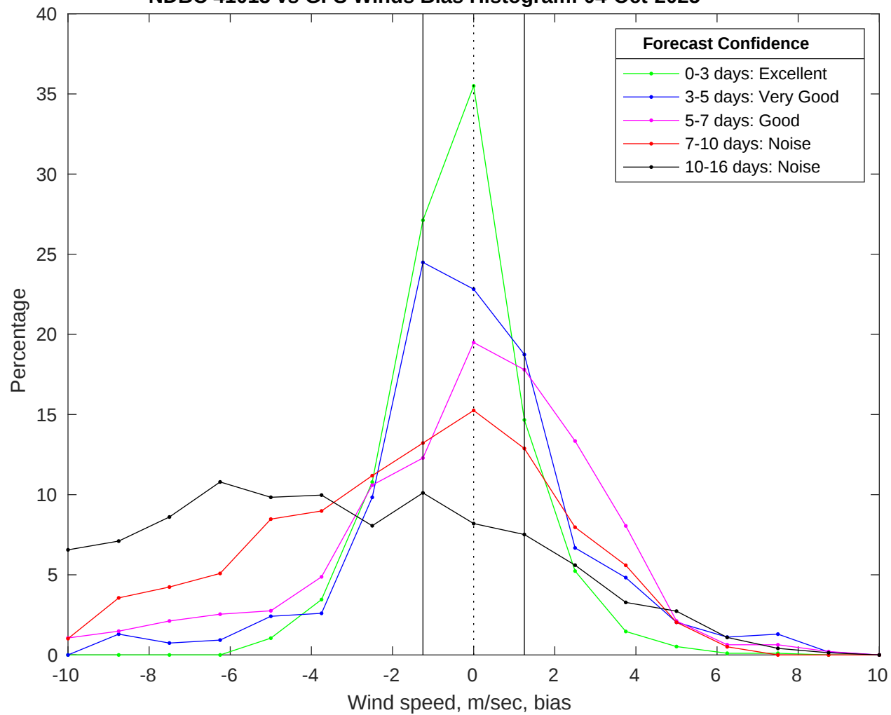
NDBC 41013 vs GFS Winds Bias Histogram: 04-Oct-2025
