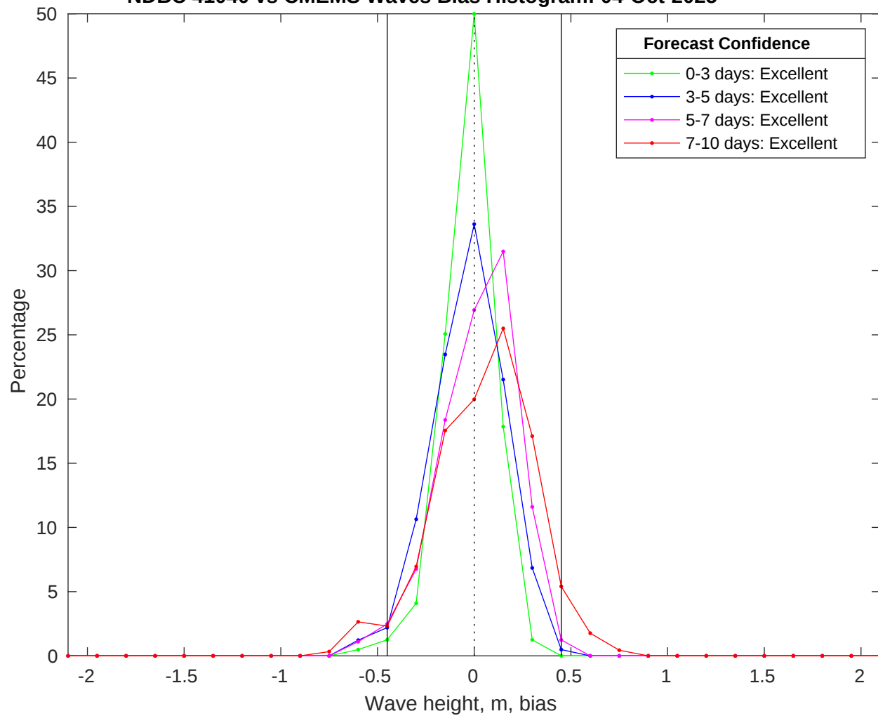
NDBC 41040 vs CMEMS Waves Bias Histogram: 04-Oct-2025
