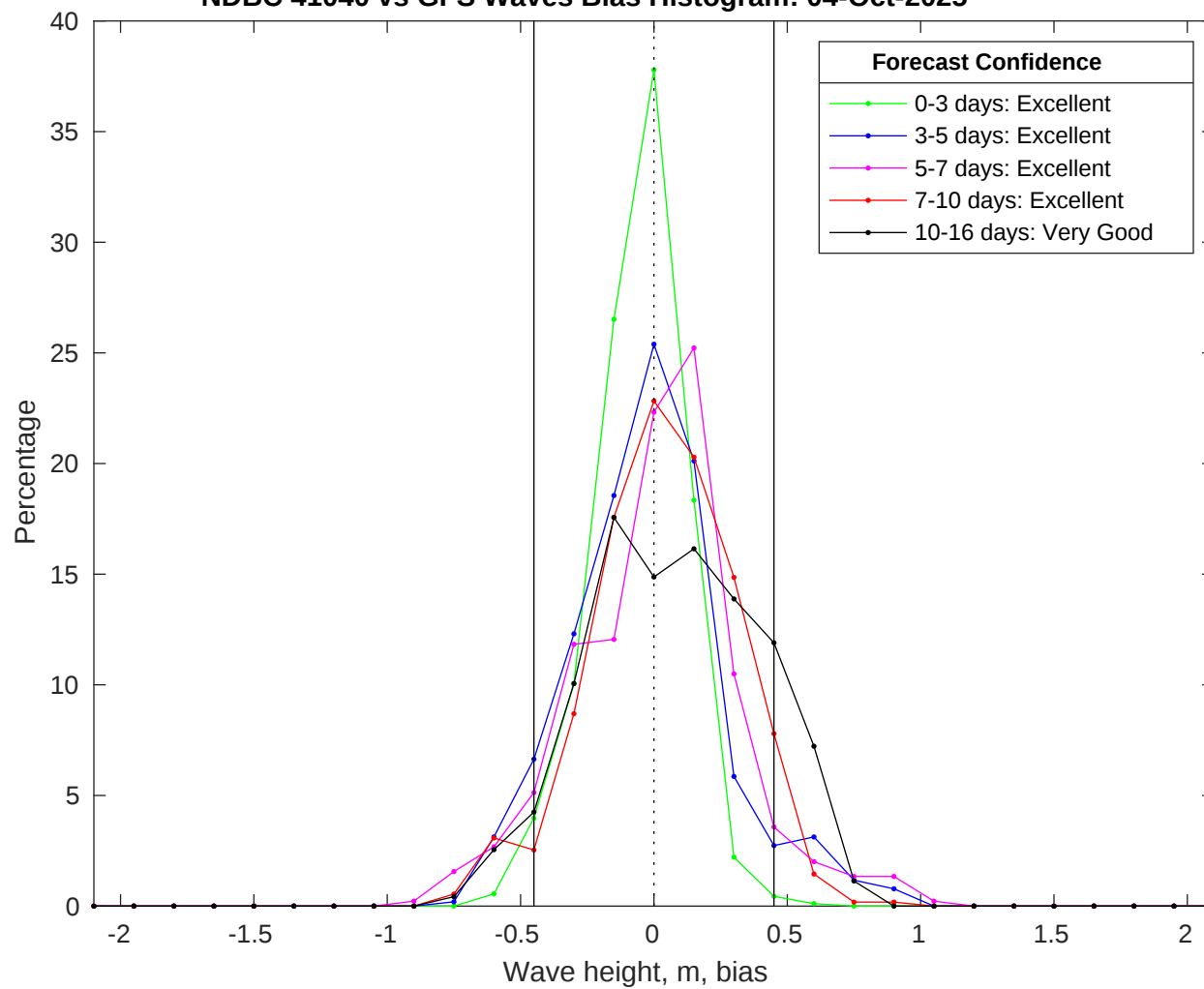
NDBC 41040 vs GFS Waves Bias Histogram: 04-Oct-2025
