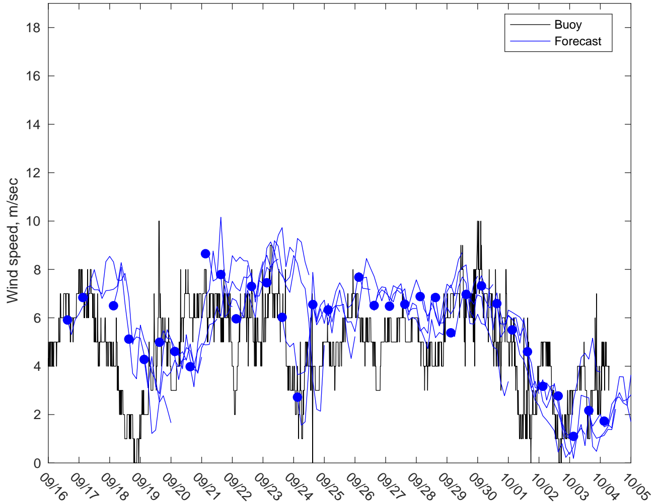
NDBC 41040 vs GFS Winds: 3 to 5 day forecast
