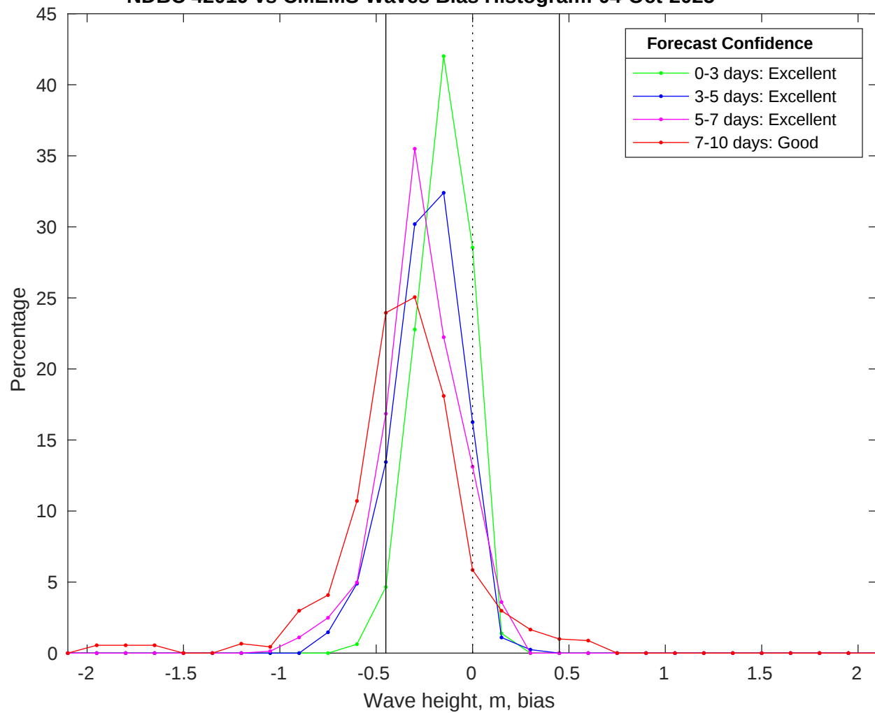
NDBC 42019 vs CMEMS Waves Bias Histogram: 04-Oct-2025
