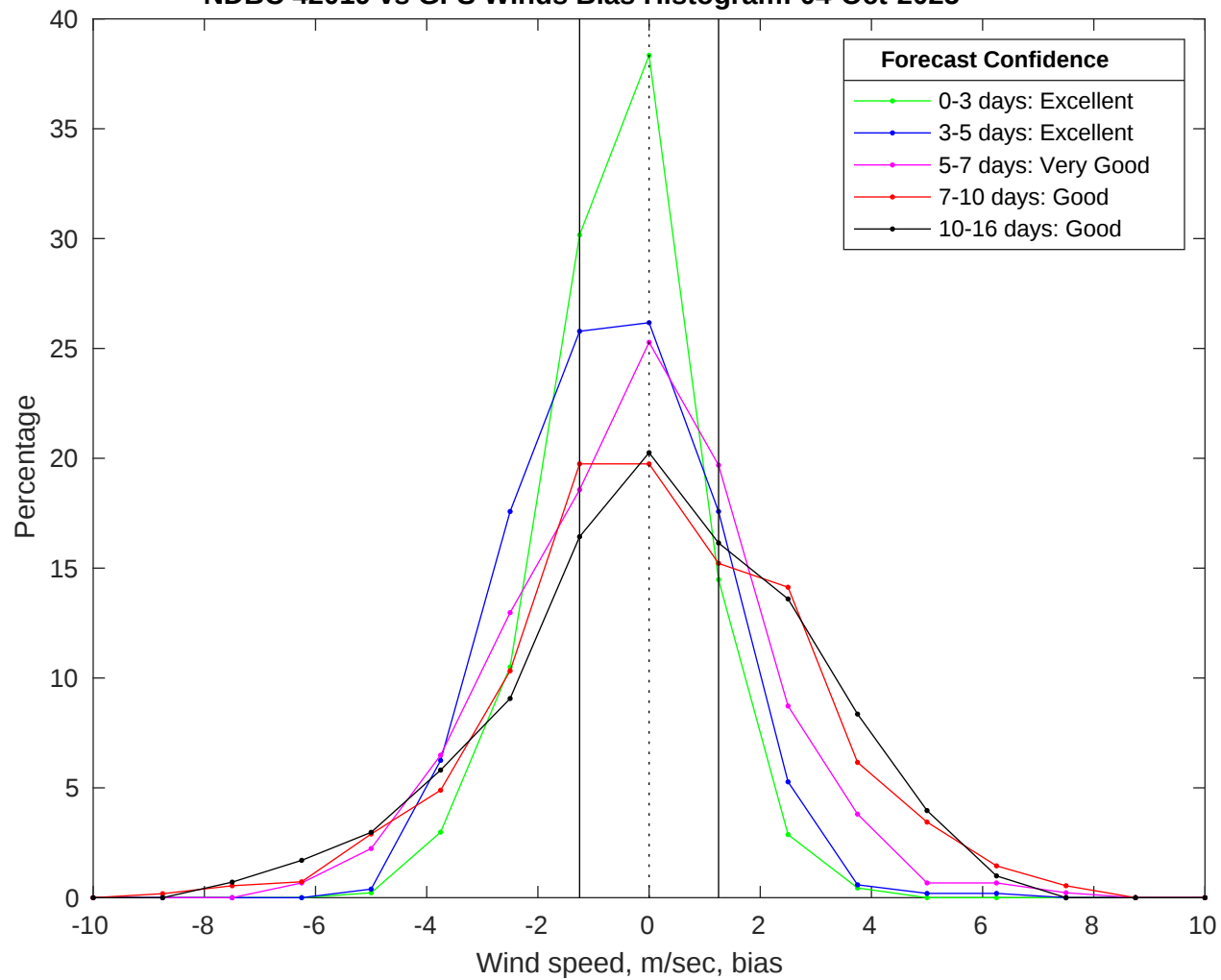
NDBC 42019 vs GFS Winds Bias Histogram: 04-Oct-2025
