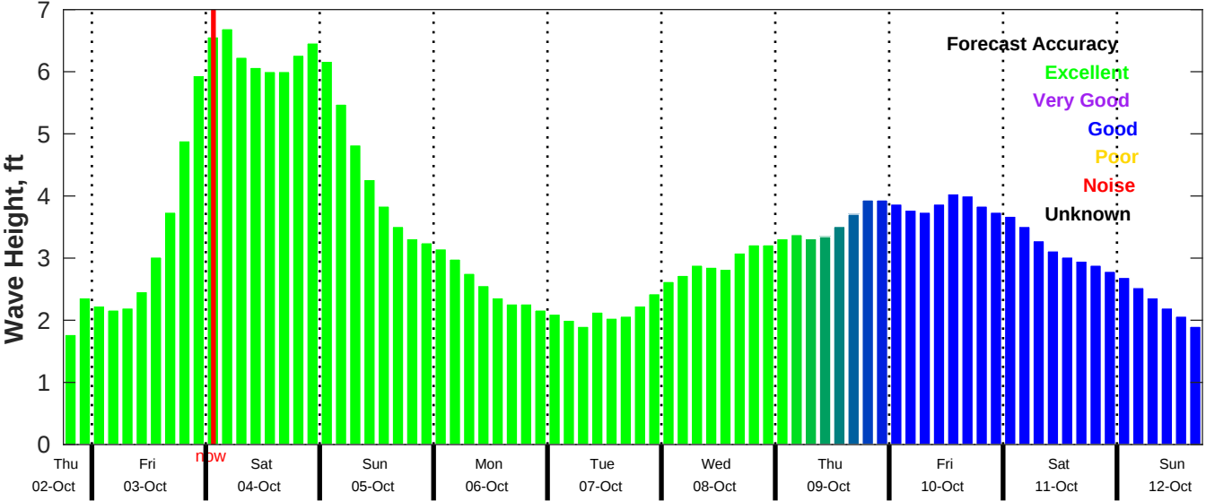
CMEMS Wave Forecast for NDBC 42019 from 02-Oct-2025 18:00:00 to 12-Oct-2025 18:00:00
