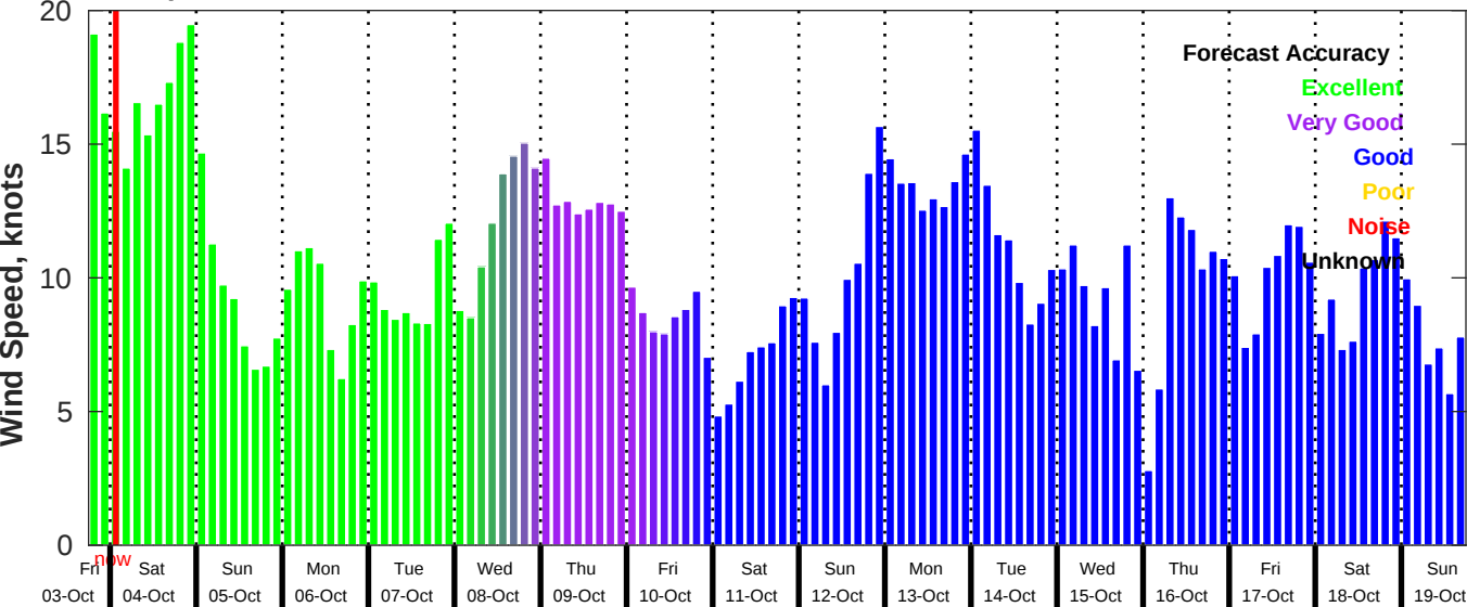
GFS Wind Speed Forecast for NDBC 42019 from 03-Oct-2025 18:00:00 to 19-Oct-2025 18:00:00
