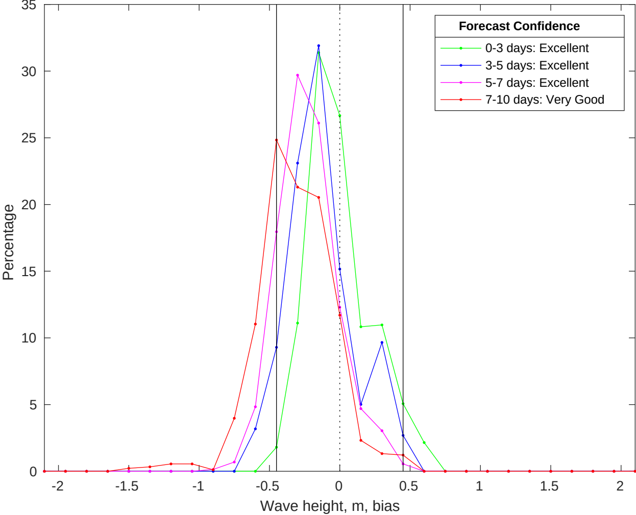
NDBC 42020 vs CMEMS Waves Bias Histogram: 04-Oct-2025
