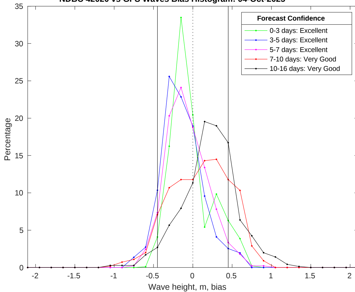
NDBC 42020 vs GFS Waves Bias Histogram: 04-Oct-2025
