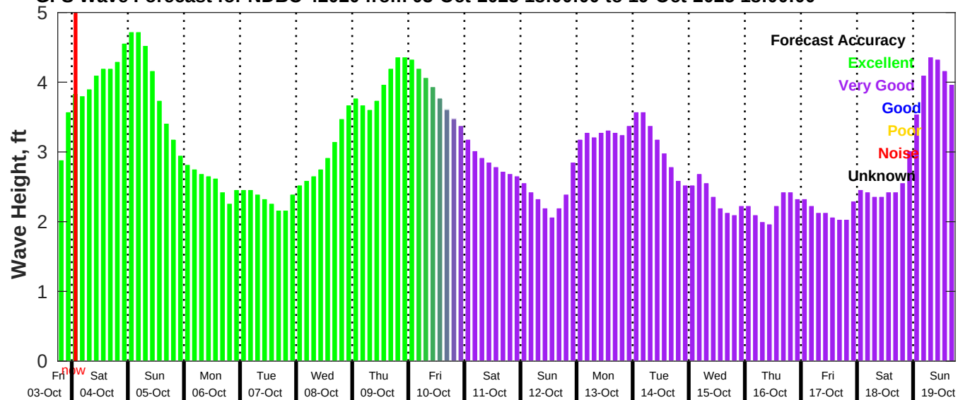
GFS Wave Forecast for NDBC 42020 from 03-Oct-2025 18:00:00 to 19-Oct-2025 18:00:00
