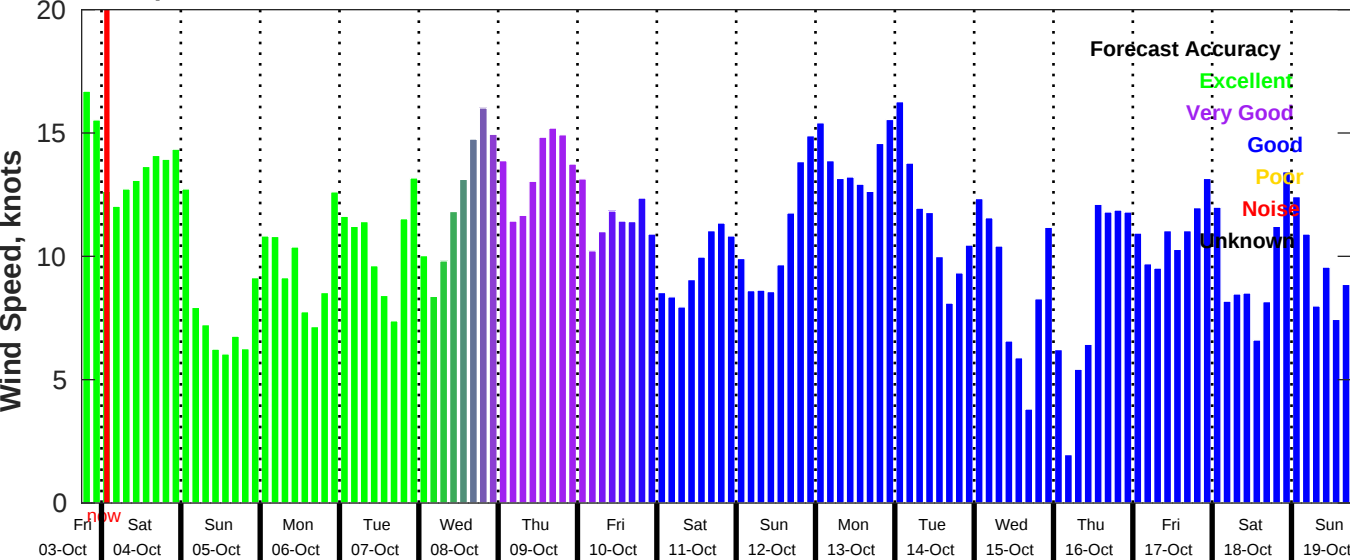
GFS Wind Speed Forecast for NDBC 42020 from 03-Oct-2025 18:00:00 to 19-Oct-2025 18:00:00
