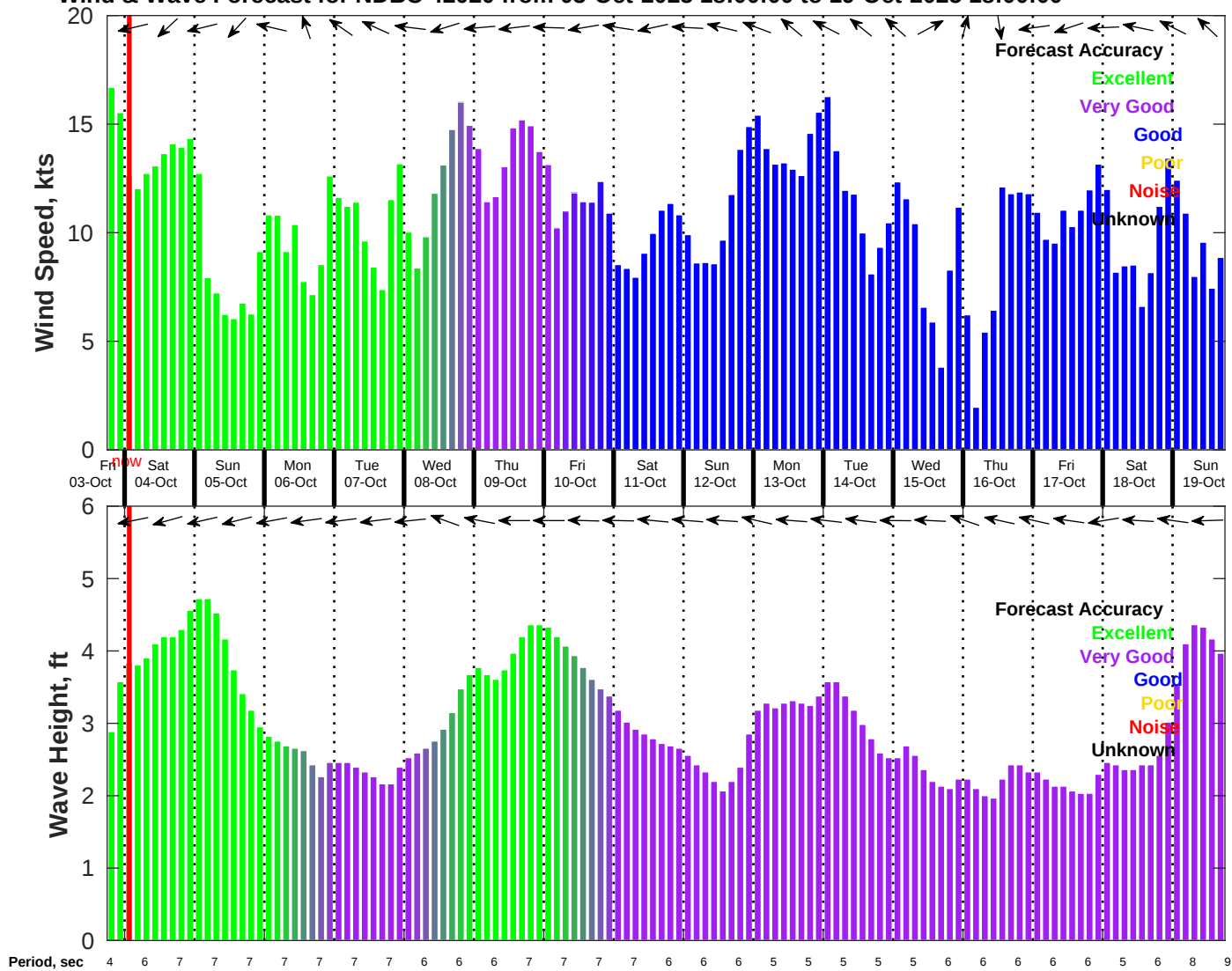
Wind & Wave Forecast for NDBC 42020 from 03-Oct-2025 18:00:00 to 19-Oct-2025 18:00:00
