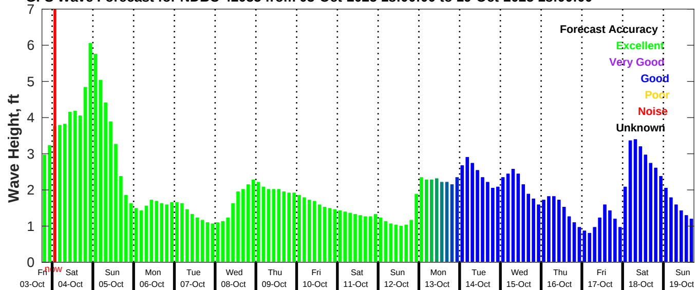
GFS Wave Forecast for NDBC 42035 from 03-Oct-2025 18:00:00 to 19-Oct-2025 18:00:00
