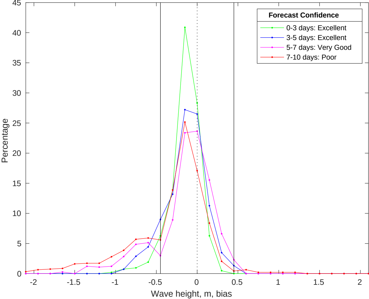
NDBC 42036 vs CMEMS Waves Bias Histogram: 04-Oct-2025
