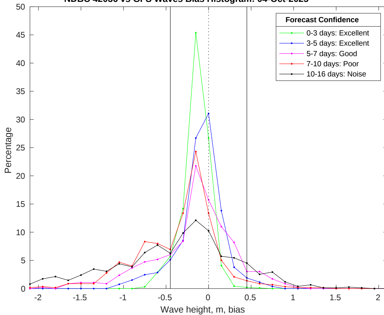
NDBC 42036 vs GFS Waves Bias Histogram: 04-Oct-2025
