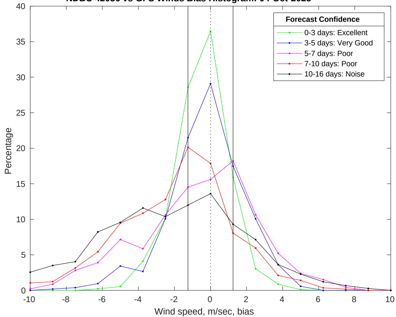
NDBC 42036 vs GFS Winds Bias Histogram: 04-Oct-2025
