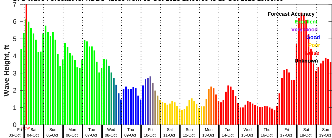
GFS Wave Forecast for NDBC 42036 from 03-Oct-2025 19:00:00 to 19-Oct-2025 19:00:00
