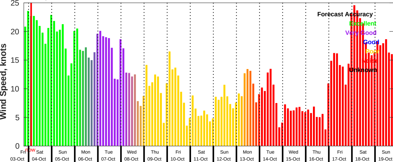
GFS Wind Speed Forecast for NDBC 42036 from 03-Oct-2025 19:00:00 to 19-Oct-2025 19:00:00
