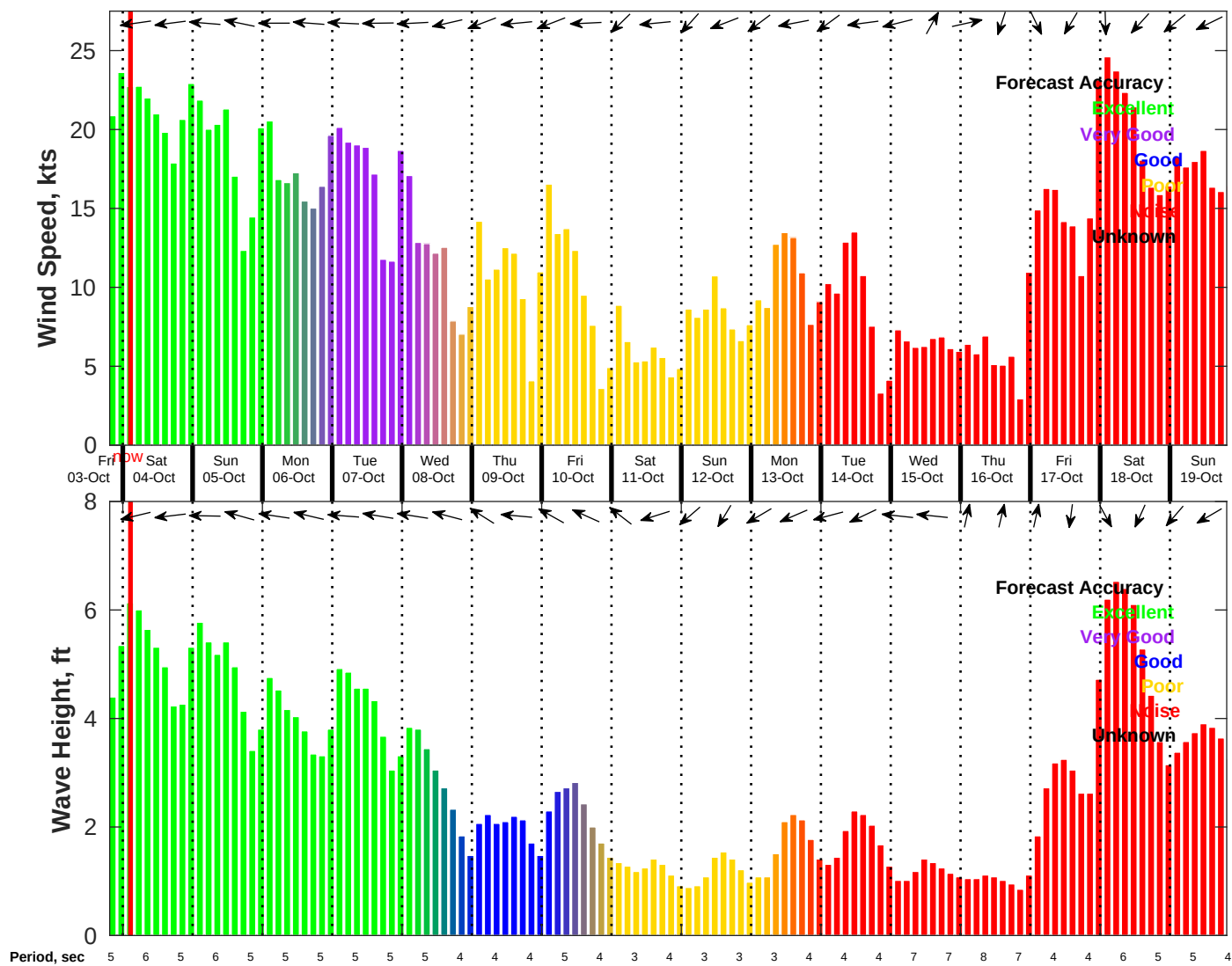
Wind & Wave Forecast for NDBC 42036 from 03-Oct-2025 19:00:00 to 19-Oct-2025 19:00:00
