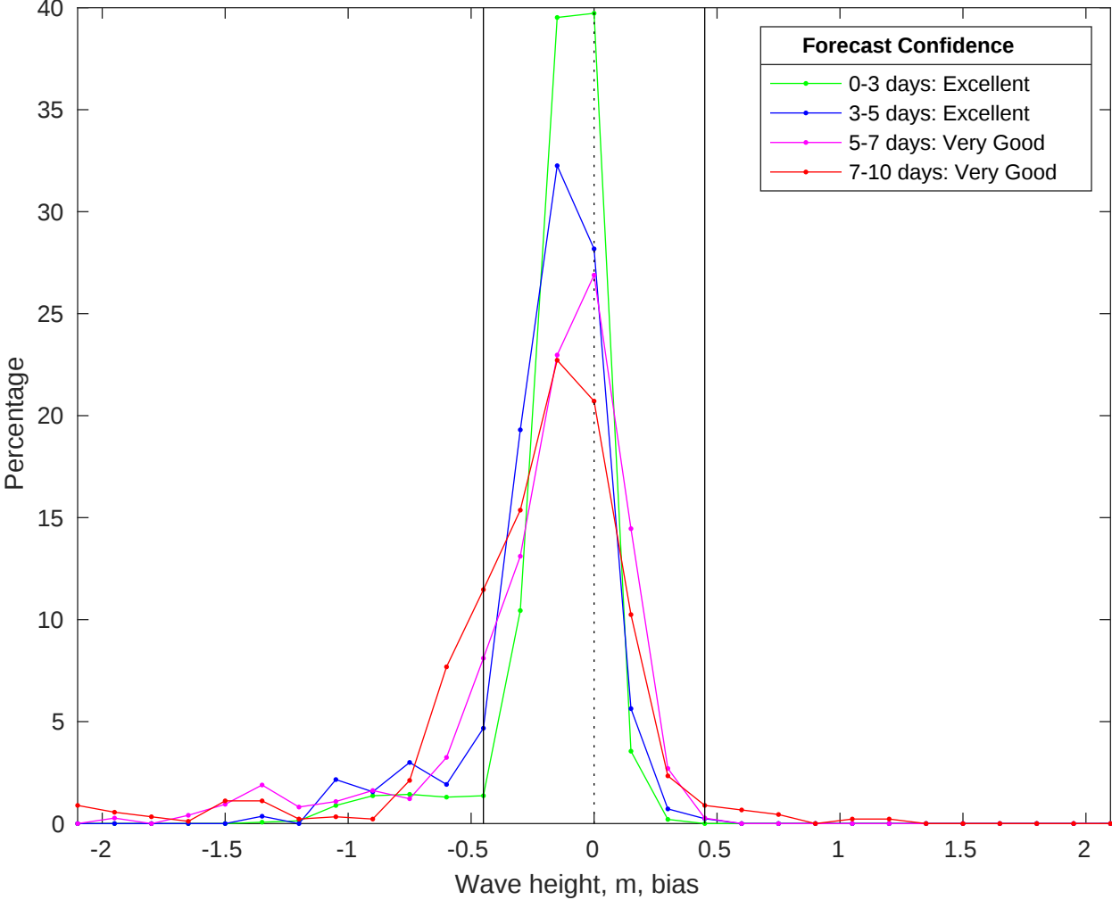
NDBC 42040 vs CMEMS Waves Bias Histogram: 04-Oct-2025
