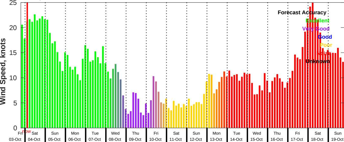
GFS Wind Speed Forecast for NDBC 42040 from 03-Oct-2025 19:00:00 to 19-Oct-2025 19:00:00
