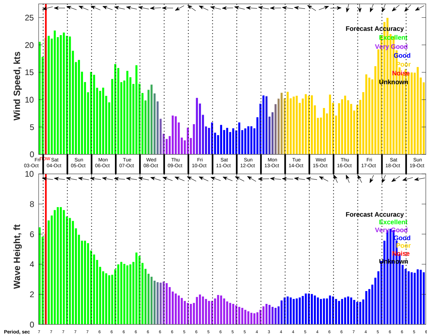
Wind & Wave Forecast for NDBC 42040 from 03-Oct-2025 19:00:00 to 19-Oct-2025 19:00:00
