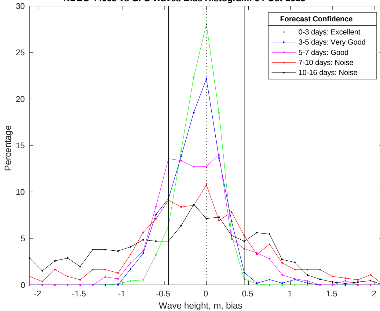
NDBC 44008 vs GFS Waves Bias Histogram: 04-Oct-2025
