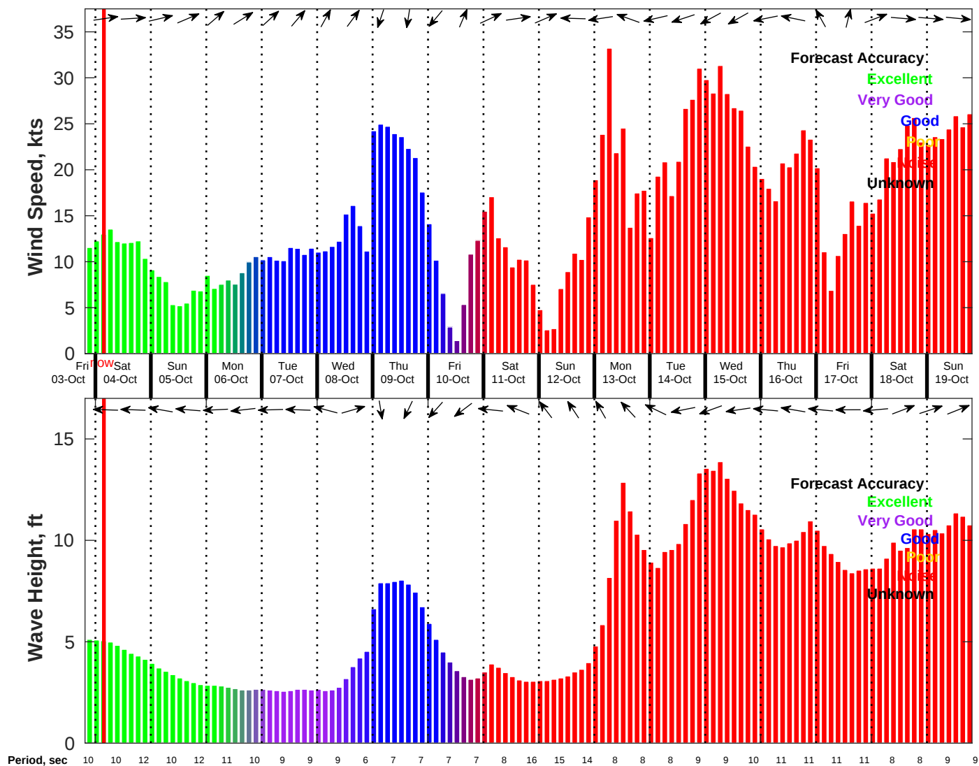
Wind & Wave Forecast for NDBC 44008 from 03-Oct-2025 20:00:00 to 19-Oct-2025 20:00:00
