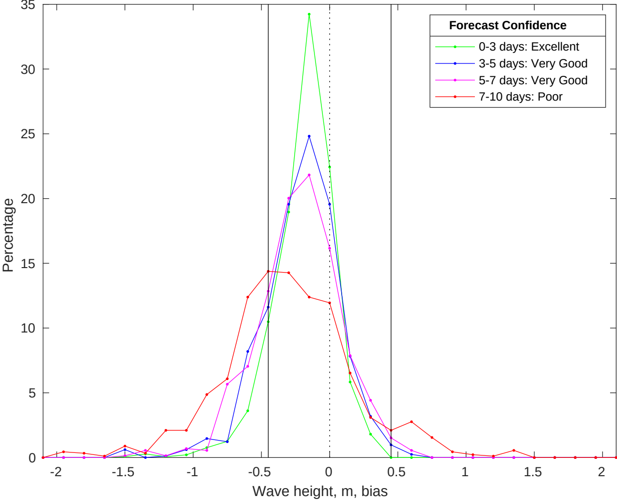
NDBC 46011 vs CMEMS Waves Bias Histogram: 04-Oct-2025
