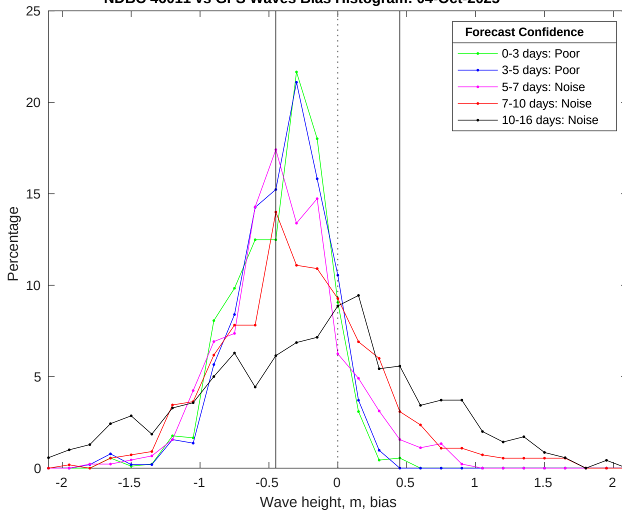
NDBC 46011 vs GFS Waves Bias Histogram: 04-Oct-2025
