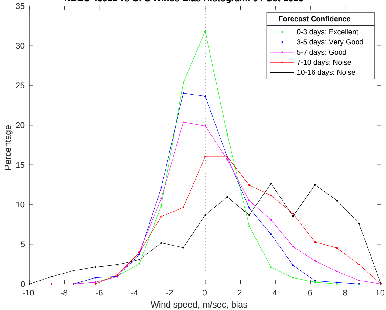
NDBC 46011 vs GFS Winds Bias Histogram: 04-Oct-2025
