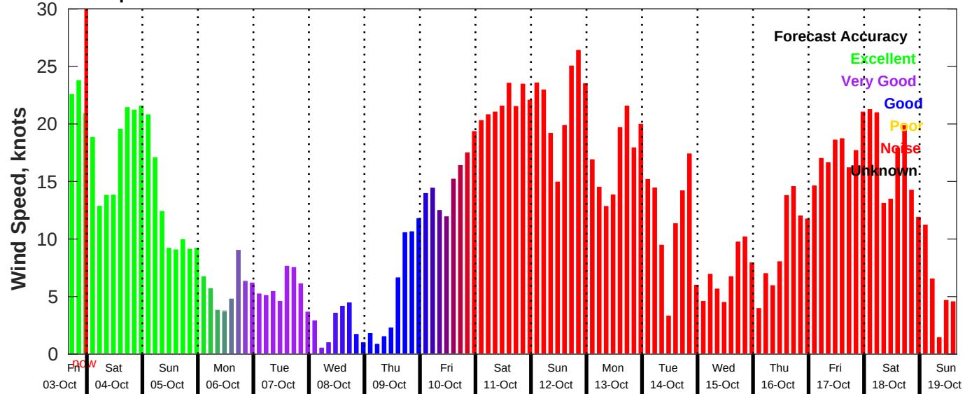
GFS Wind Speed Forecast for NDBC 46011 from 03-Oct-2025 16:00:00 to 19-Oct-2025 16:00:00
