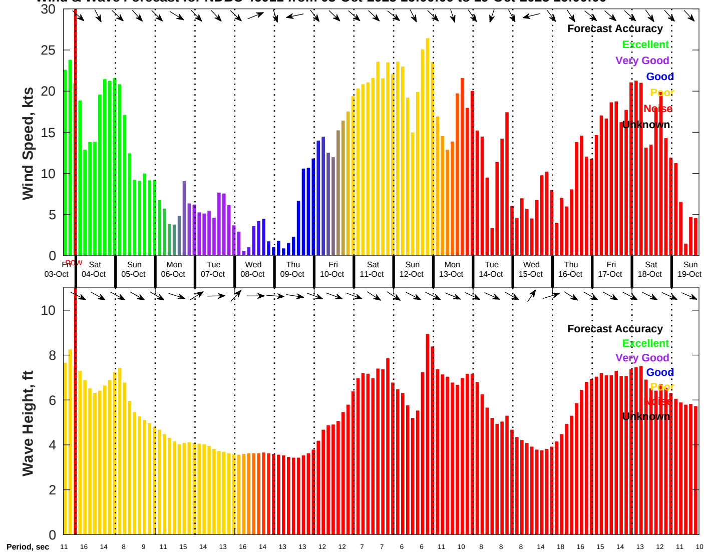
Wind & Wave Forecast for NDBC 46011 from 03-Oct-2025 16:00:00 to 19-Oct-2025 16:00:00
