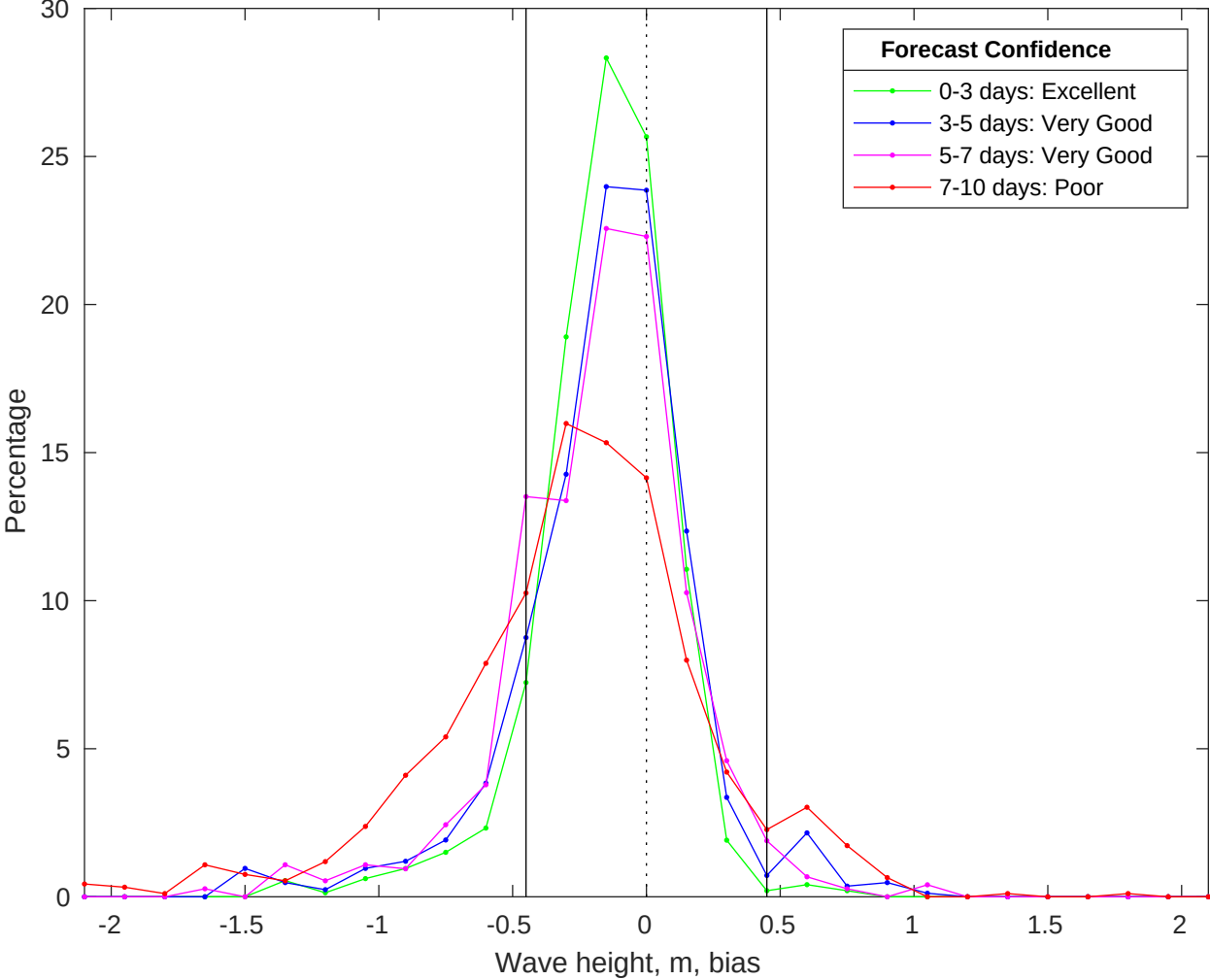
NDBC 46028 vs CMEMS Waves Bias Histogram: 04-Oct-2025
