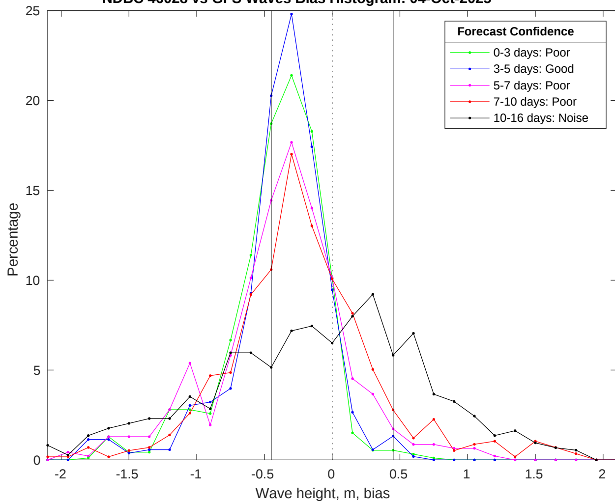
NDBC 46028 vs GFS Waves Bias Histogram: 04-Oct-2025
