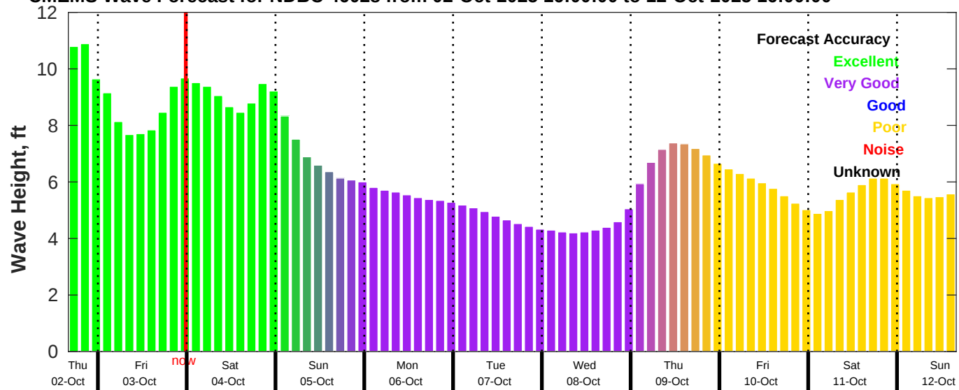
CMEMS Wave Forecast for NDBC 46028 from 02-Oct-2025 16:00:00 to 12-Oct-2025 16:00:00
