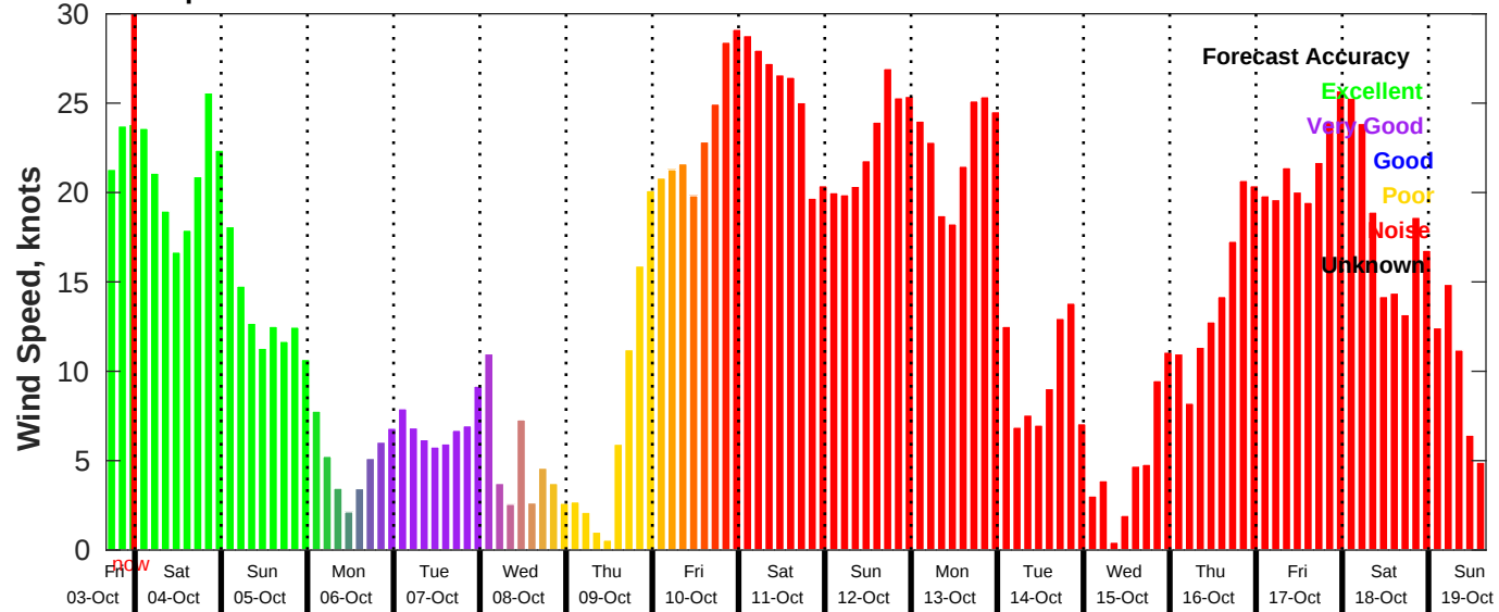
GFS Wind Speed Forecast for NDBC 46028 from 03-Oct-2025 16:00:00 to 19-Oct-2025 16:00:00
