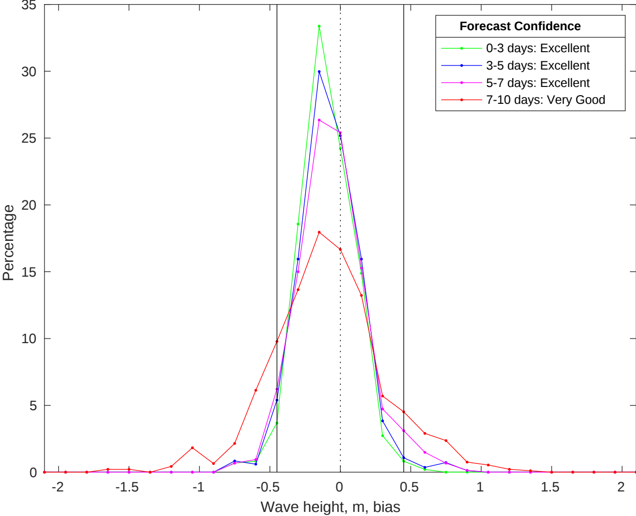
NDBC 46054 vs CMEMS Waves Bias Histogram: 04-Oct-2025
