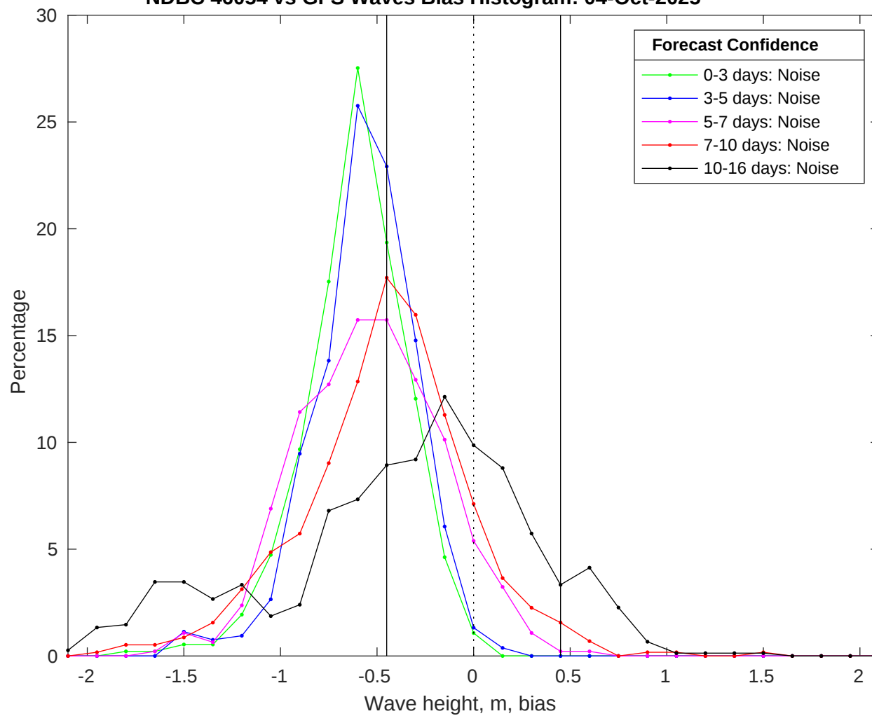
NDBC 46054 vs GFS Waves Bias Histogram: 04-Oct-2025
