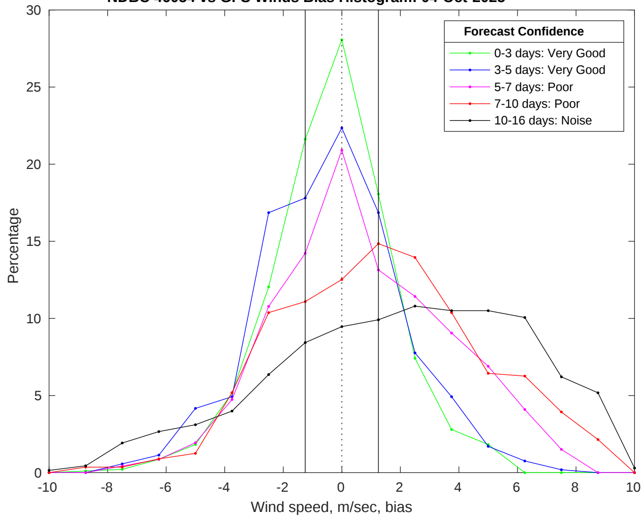
NDBC 46054 vs GFS Winds Bias Histogram: 04-Oct-2025
