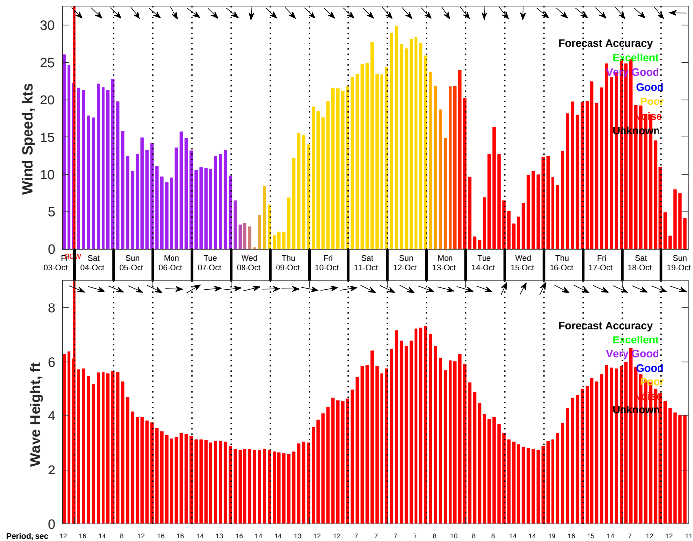
Wind & Wave Forecast for NDBC 46054 from 03-Oct-2025 16:00:00 to 19-Oct-2025 16:00:00
