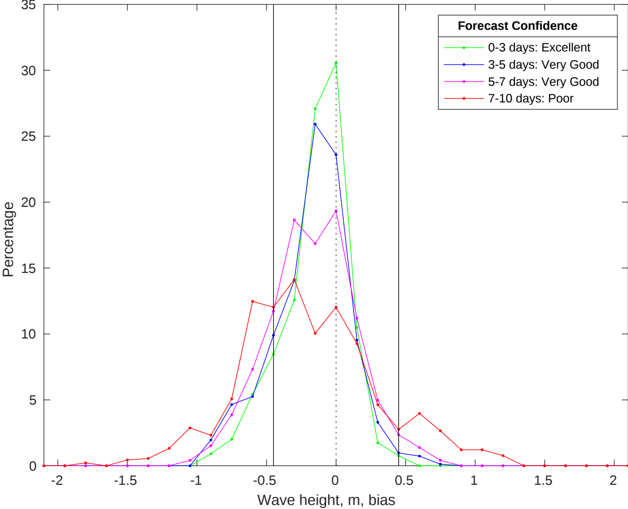
NDBC 46069 vs CMEMS Waves Bias Histogram: 04-Oct-2025
