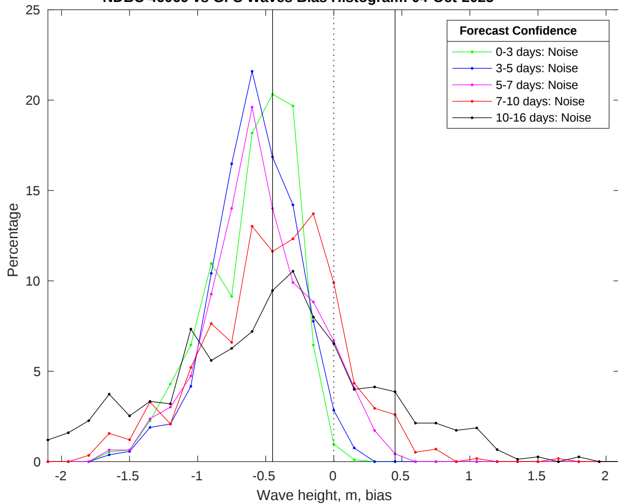
NDBC 46069 vs GFS Waves Bias Histogram: 04-Oct-2025
