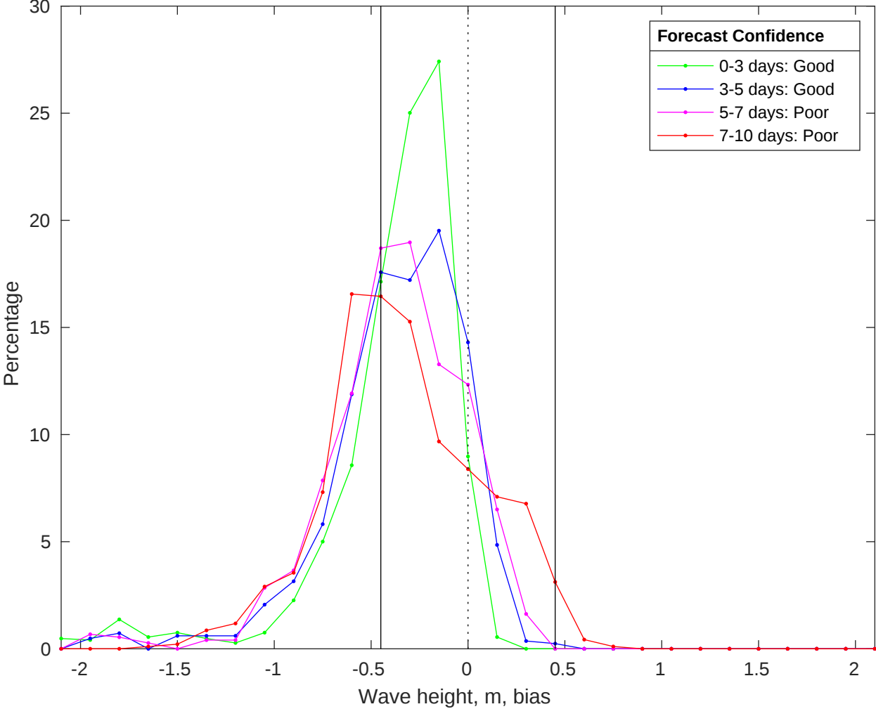
NDBC 51209 vs CMEMS Waves Bias Histogram: 04-Oct-2025
