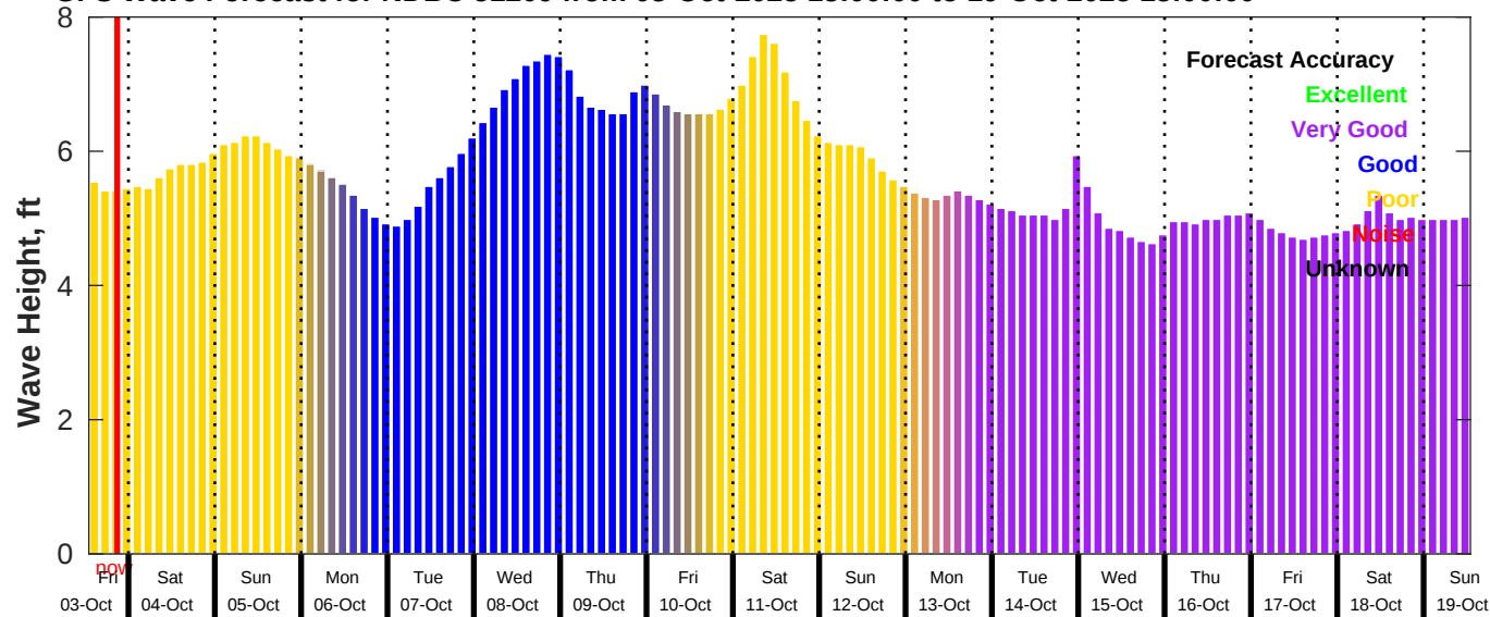
GFS Wave Forecast for NDBC 51209 from 03-Oct-2025 13:00:00 to 19-Oct-2025 13:00:00
