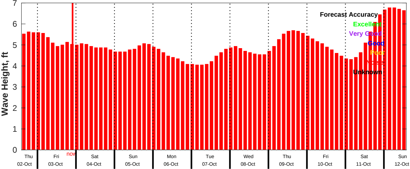
CMEMS Wave Forecast for NDBC 51211 from 02-Oct-2025 14:00:00 to 12-Oct-2025 14:00:00
